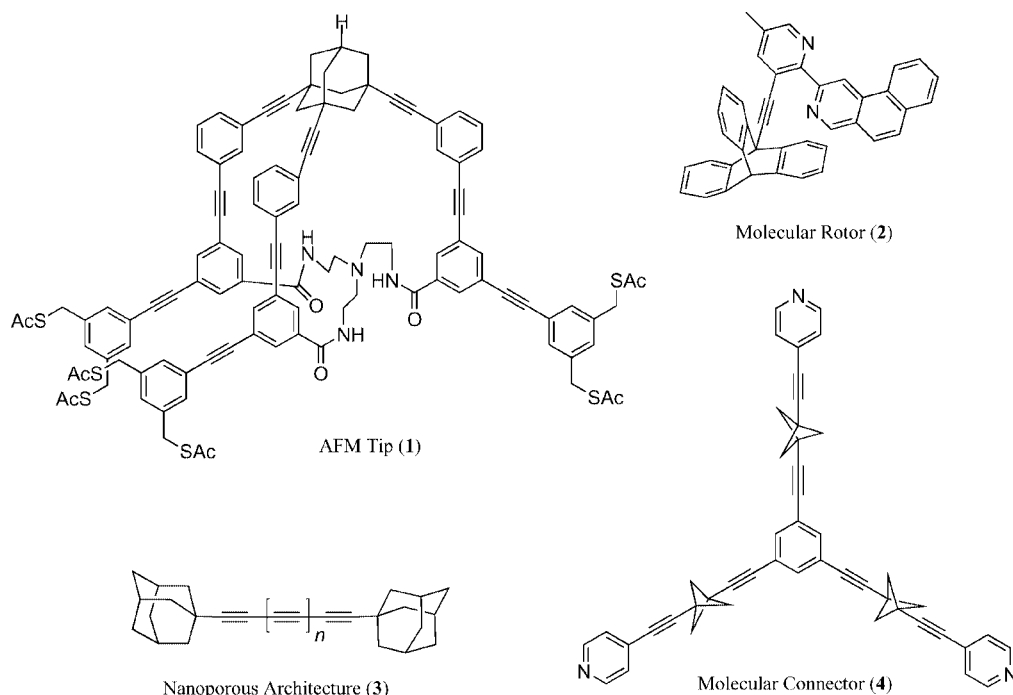
Figure 1. Examples of an AFM tip (1), molecular rotor (2), nanoporous architecture (3) and a molecular connector (4) containing bridgehead acetylenic bonds.
