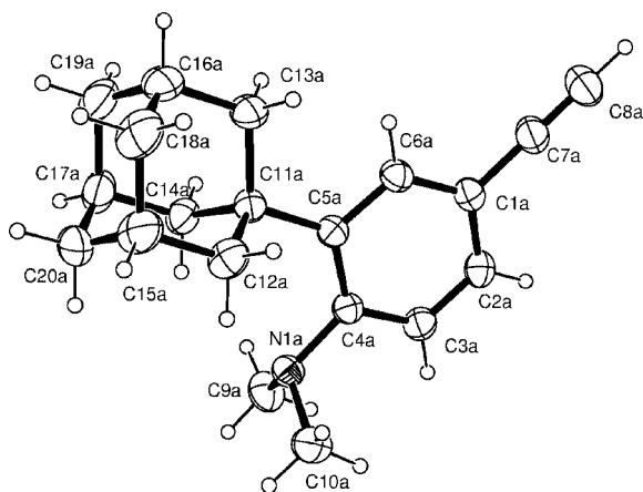
Figure 2. ORTEP3 drawing of compound 15 (30% probability ellipsoids).
